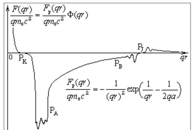
图一 天体运行轨道背景介质理论的作用力趋势曲线图 Fig.1 The interaction tendency curve in the background medium theory of celestial body motion orbit
